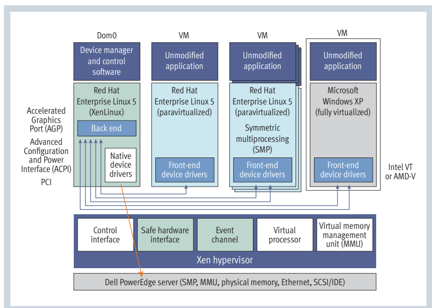
Figure 1. Xen hypervisor architecture
