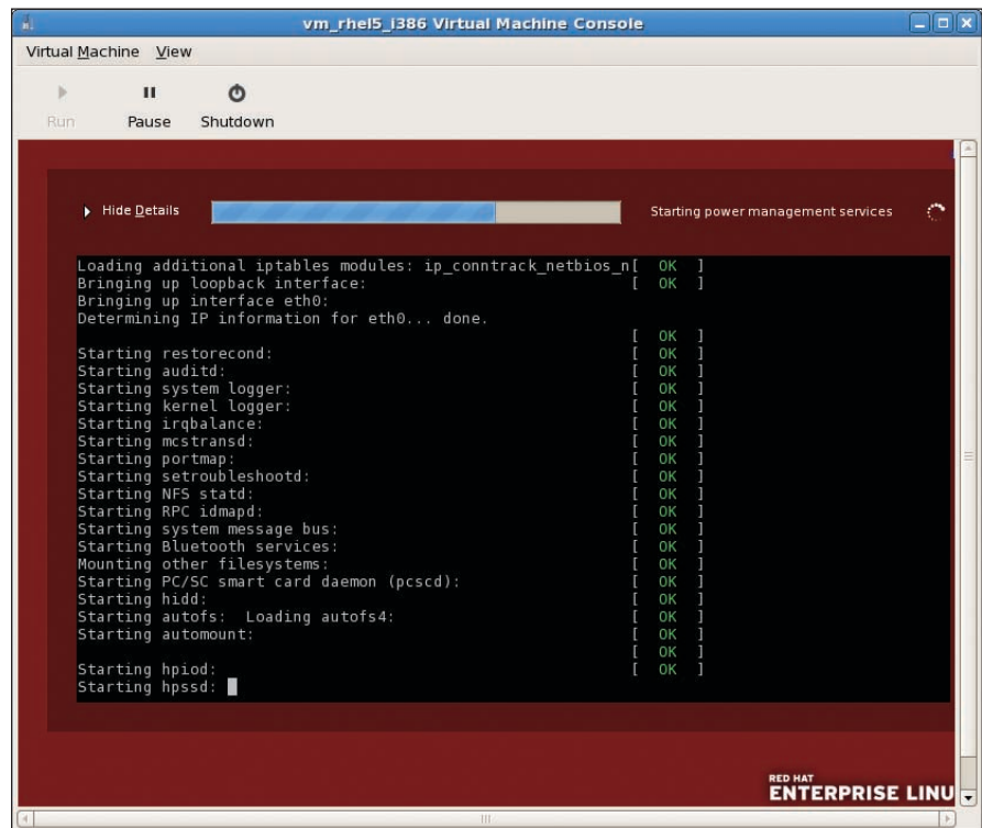
Figure 6. Virtual machine booting in Red Hat Enterprise Linux 5
