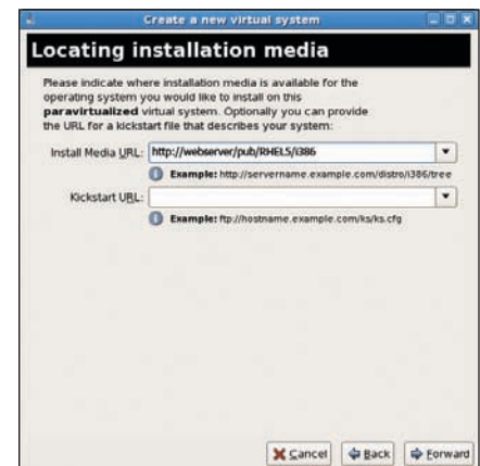
Figure 2. “Locating installation media” step when creating a virtual machine in Red Hat Enterprise Linux 5 Virtual Machine Manager
